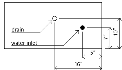
water connections
